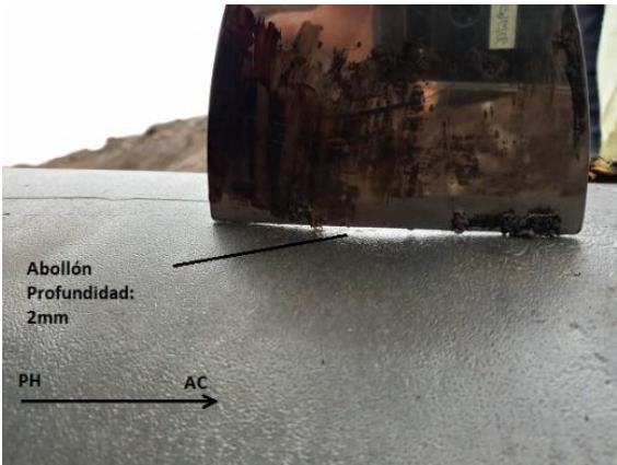
FIGURE 10 – damage assessment. – Source: Athor of the paper
