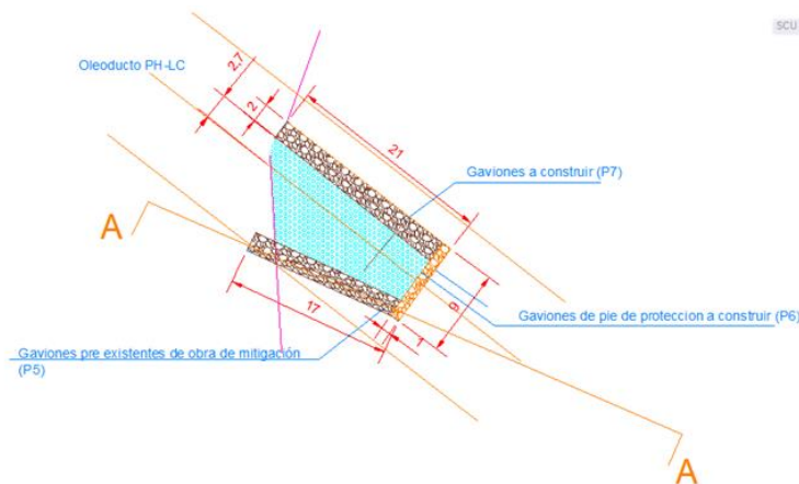
FIGURE 14 – Schematic plan of the final provisional work – Source: Author of the paper
