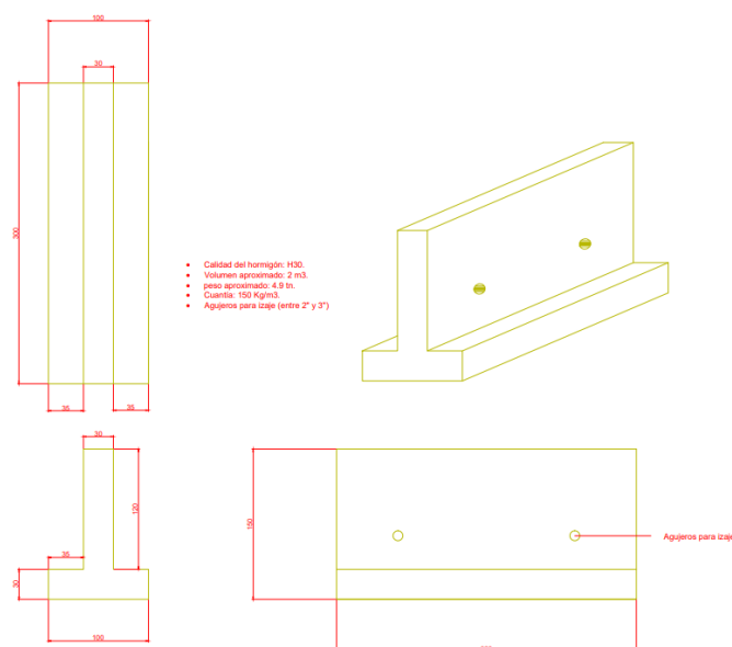
FIGURE 17 -Sleepers Plans – Source: Author of the paper
