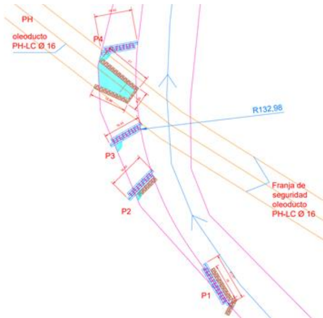
FIGURE 23 – General Implementation of Protections - Source: Author of the paper
