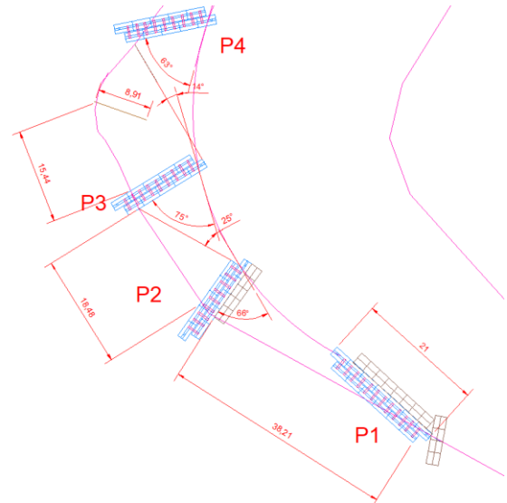
FIGURE 24 – General implementation of protections with indication of main angles and distances - Source: Autor of the paper
