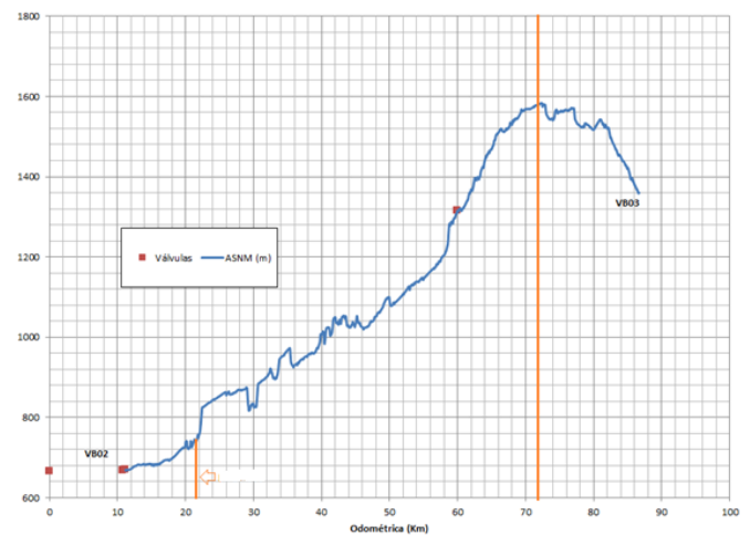
FIGURE 13 – Altimetry between VB – Source: Authr of the paper.
