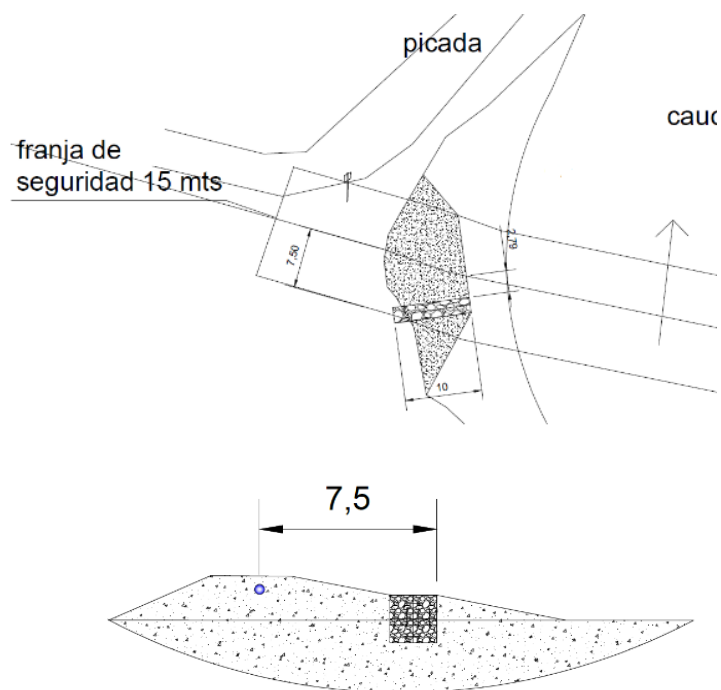
FIGURE 13 – Provisional work schematic plan – Source: Author of the paper
